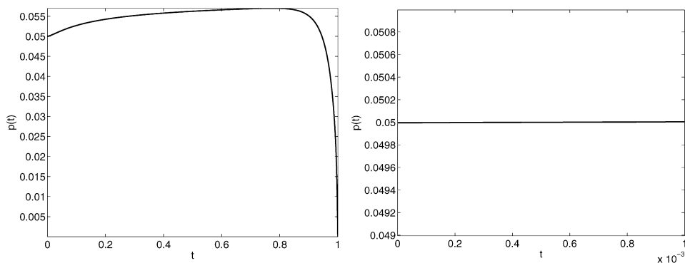
Fig. 2. Numerical solution of (4.3)–(4.5) for a_0 = 2 , b_0 = 3 , \gamma = 1.8 . Left graph: p(t) , t \in [0, 1] ; right graph: p(t) , t \in [0, 10^{-3}] .
