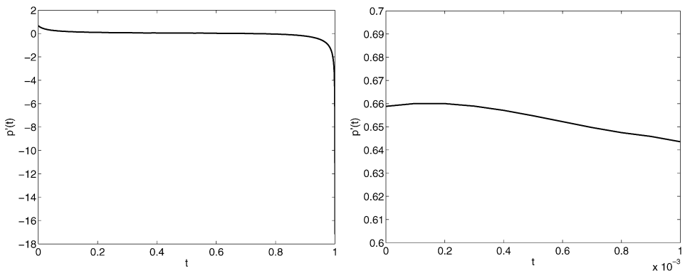
Fig. 5. Derivative of the numerical solution of (4.3)–(4.5) for a_0 = 1 , b_0 = 2 , \gamma = \frac{3}{2} . Left graph: p'(t) , t \in [0, 1] ; right graph: p'(t) , t \in [0, 10^{-3}] .
