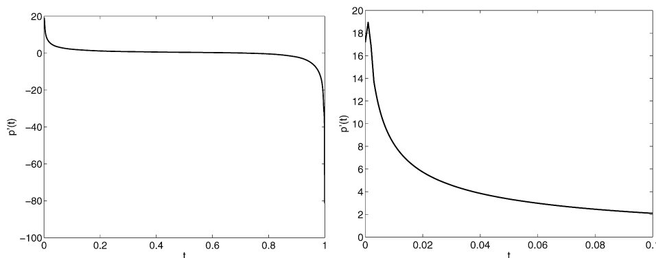
Fig. 7. Derivative of the numerical solution of (4.3)–(4.5) for a_0 = 1 , b_0 = 2 , \gamma = 1.4 . Left graph: p'(t) , t \in [0, 1] ; right graph: p'(t) , t \in [0, 10^{-1}] .
