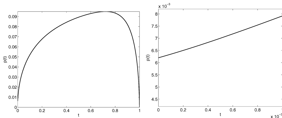
Fig. 6. Numerical solution of (4.3)–(4.5) for a_0 = 1 , b_0 = 2 , \gamma = 1.4 . Left graph: p(t) , t \in [0, 1] ; right graph: p(t) , t \in [0, 10^{-3}] .
