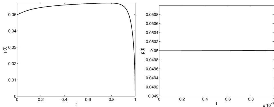
Fig. 1. Numerical solution of (4.1), (4.2) for a_0 = 2 , b_0 = 3 , \gamma = 1.8 . Left graph: p(t) , t \in [0, 1] ; right graph: p(t) , t \in [0, 10^{-3}] .
