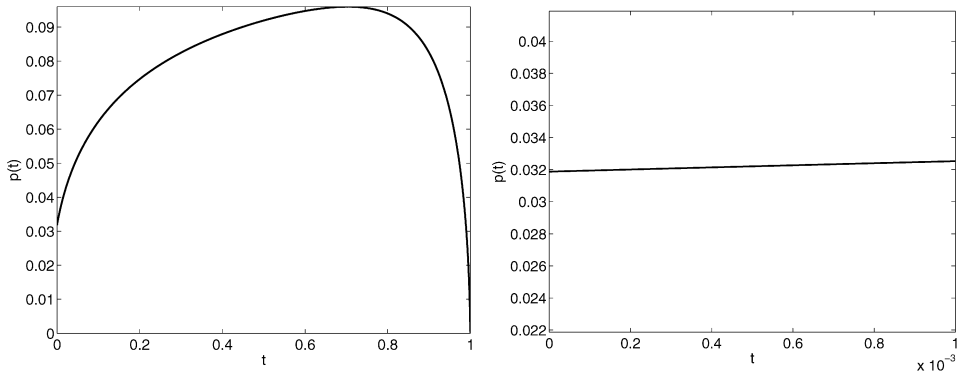
Fig. 4. Numerical solution of (4.3)–(4.5) for a_0 = 1 , b_0 = 2 , \gamma = \frac{3}{2} . Left graph: p(t) , t \in [0, 1] ; right graph: p(t) , t \in [0, 10^{-3}] .
